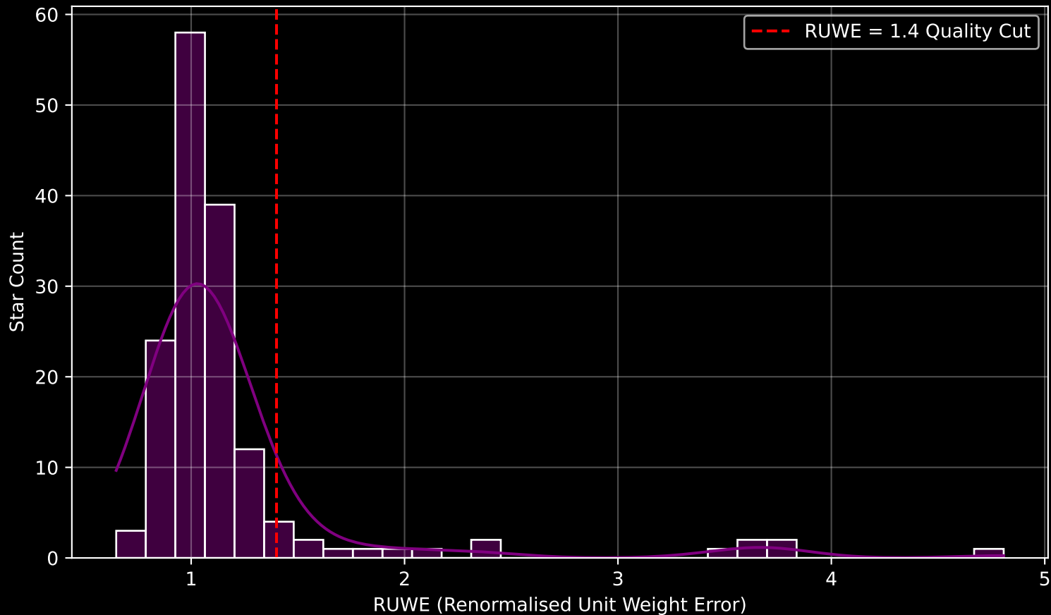
GAPOGEE DR17 Field [287-34-O_TESS] RUWE Distribution (n= 154)
