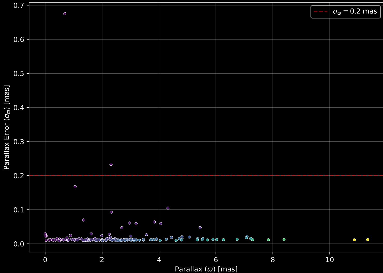
APOGEE DR17 Field: [287-34-O_TESS] Parallax Quality (n= 159)
