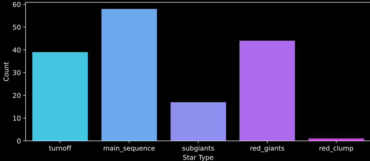
APOGEE DR17 Field: [287-34-O_TESS] Count plot of Star Type
